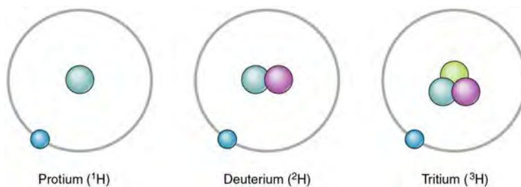
Figure 2.5 Isotopes of Hydrogen Protium, designated ^1\text{H} , has one proton and no neutrons. It is by far the most abundant isotope of hydrogen in nature. Deuterium, designated ^2\text{H} , has one proton and one neutron. Tritium, designated ^3\text{H} , has two neutrons.
