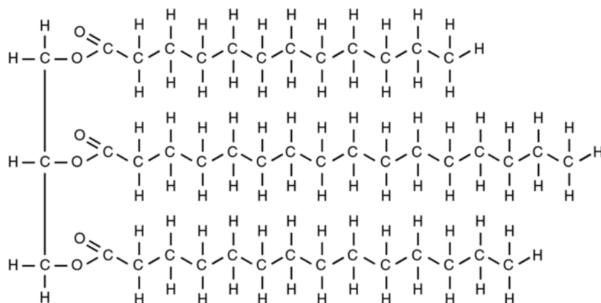
(a) Triglyceride
